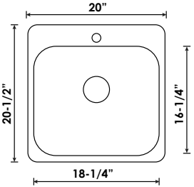
B203 TOP-MOUNT TRADITIONAL SINGLE HOLE, 18 GAUGE SINK 20" x 20 1/2" x 10" - Minimum Cabinet Size: 21"
