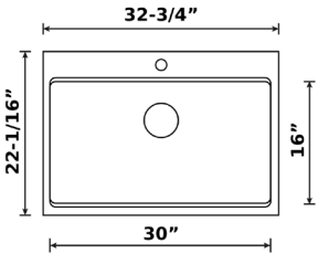
B1251 STAINLESS WORKSTATION TOP-MOUNT 18 GAUGE, 10 MM RADIUS SINK 32 3/4" x 22 1/16" x 9" - Minimum Cabinet Size: 34"
