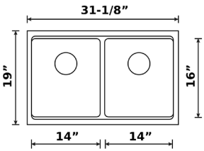
B1861 LOW DIVIDE STAINLESS WORKSTATION UNDER-MOUNT 18 GAUGE, 10 MM RADIUS SINK 31 1/8" x 19" x 9 1/4" x 9 1/4" - Minimum Cabinet Size: 33"
