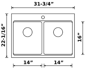
B1261 LOW DIVIDE STAINLESS WORKSTATION TOP-MOUNT 18 GAUGE, 10 MM RADIUS SINK 31 3/4" x 22 1/16" x 9" x 9" - Minimum Cabinet Size: 33"
