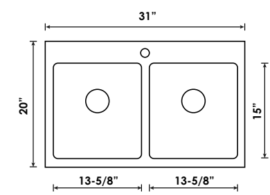
B1208 TOP-MOUNT SINGLE HOLE 18 GAUGE, 10MM RADIUS SINK 31" x 20" x 10" - Minimum Cabinet Size: 32"
